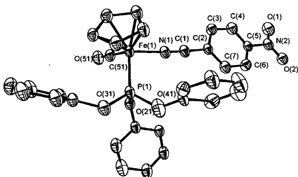
Fig. 2. ORTEP diagram for [Fe(\eta^5-C_5H_5)(CO)(P(OC_6H_5)_3)(p-NCC_6H_4NO_2)]^+ , with 20% thermal ellipsoids, showing the atomic labelling scheme. Hydrogen atoms have been omitted for clarity.
