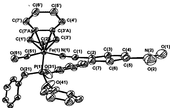
Fig. 3. ORTEP diagram for [Fe(\eta^5-C_9H_7)(CO)(P(OC_6H_5)_3)(p-NCC_6H_4NO_2)]^+ , with 20% thermal ellipsoids, showing the atomic labelling scheme. Hydrogen atoms have been omitted for clarity.
